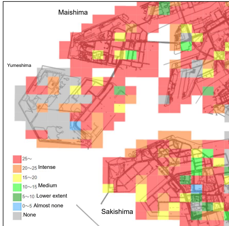
Figure 4. Liquefaction prediction map in the major Nankai Trough Earthquake 5
